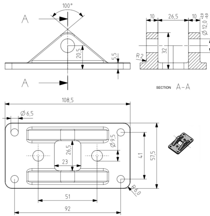
Optional replacement Rudder Gudgeon
