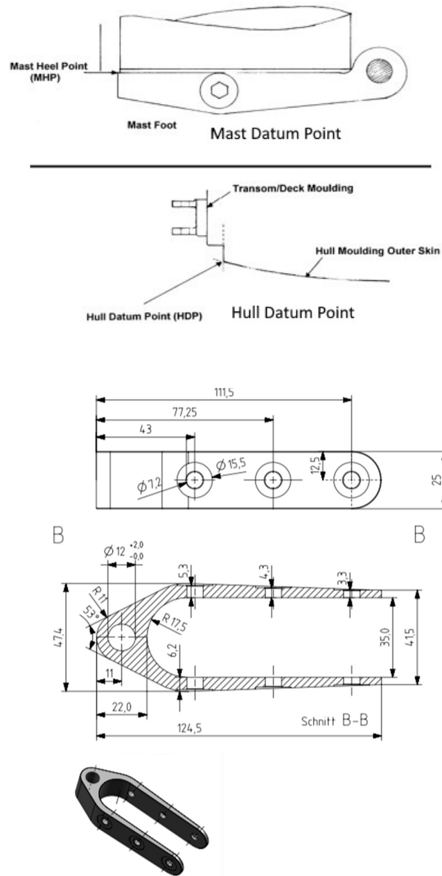
Optional replacement Rudder Fitting
