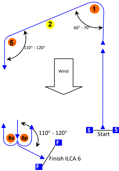
ILCA 6 START -1 – 2 –5 – 6S/6P -5 – 6p – FINISH
